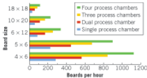
Figure 1. Throughput capability of a batch-format defluxing system.
